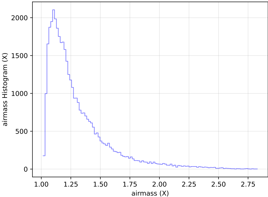
weather_cloudso18v3.4_10yrs Yr 1 y band: airmass Histogram
