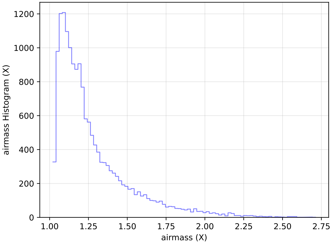
weather_cloudso18v3.4_10yrs Yr 1 u band: airmass Histogram
