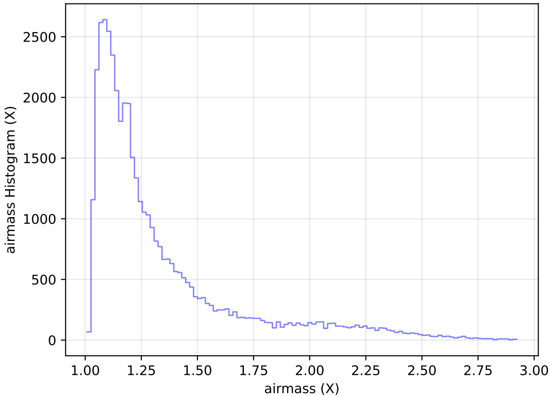
weather_cloudso18v3.4_10yrs Yr 1 i band: airmass Histogram
