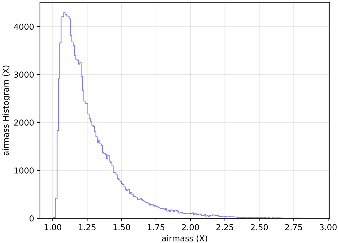
weather_cloudso18v3.4_10yrs WFD u band: airmass Histogram
