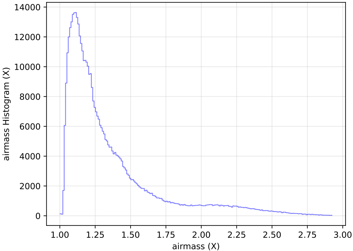
weather_cloudso18v3.4_10yrs All sky z band: airmass Histogram
