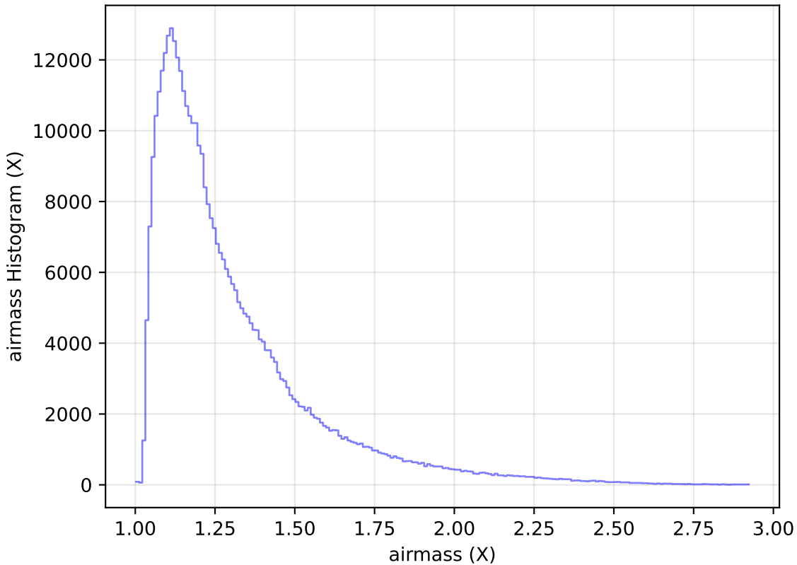
weather_cloudso18v3.4_10yrs All sky y band: airmass Histogram
