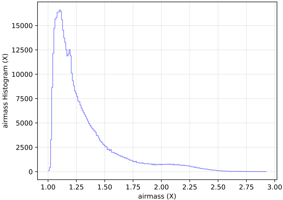
weather_cloudso18v3.4_10yrs All sky r band: airmass Histogram
