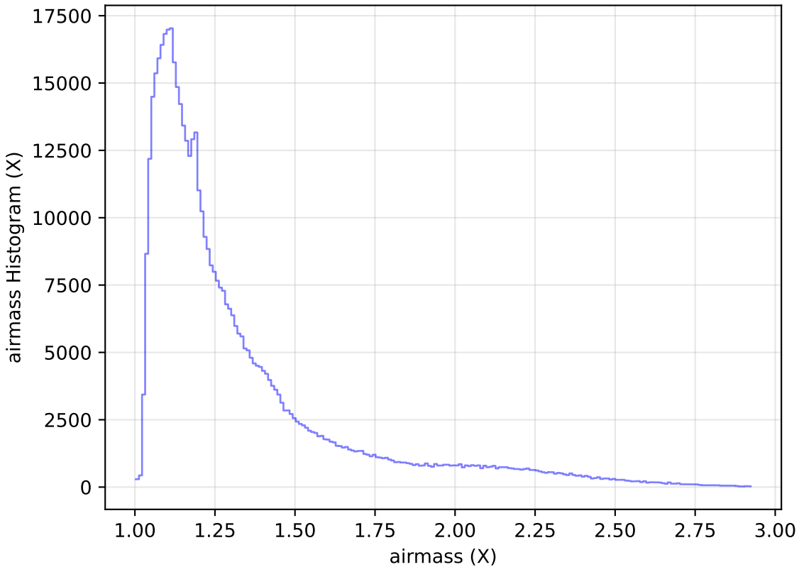
weather_cloudso18v3.4_10yrs All sky i band: airmass Histogram
