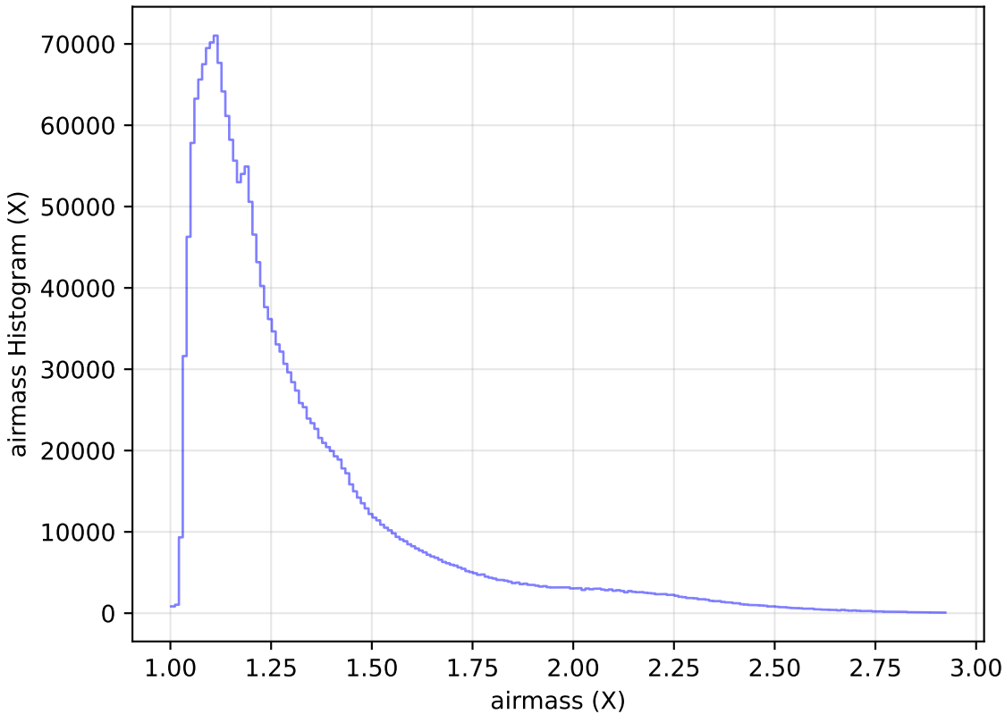
weather_cloudso18v3.4_10yrs All sky all bands: airmass Histogram
