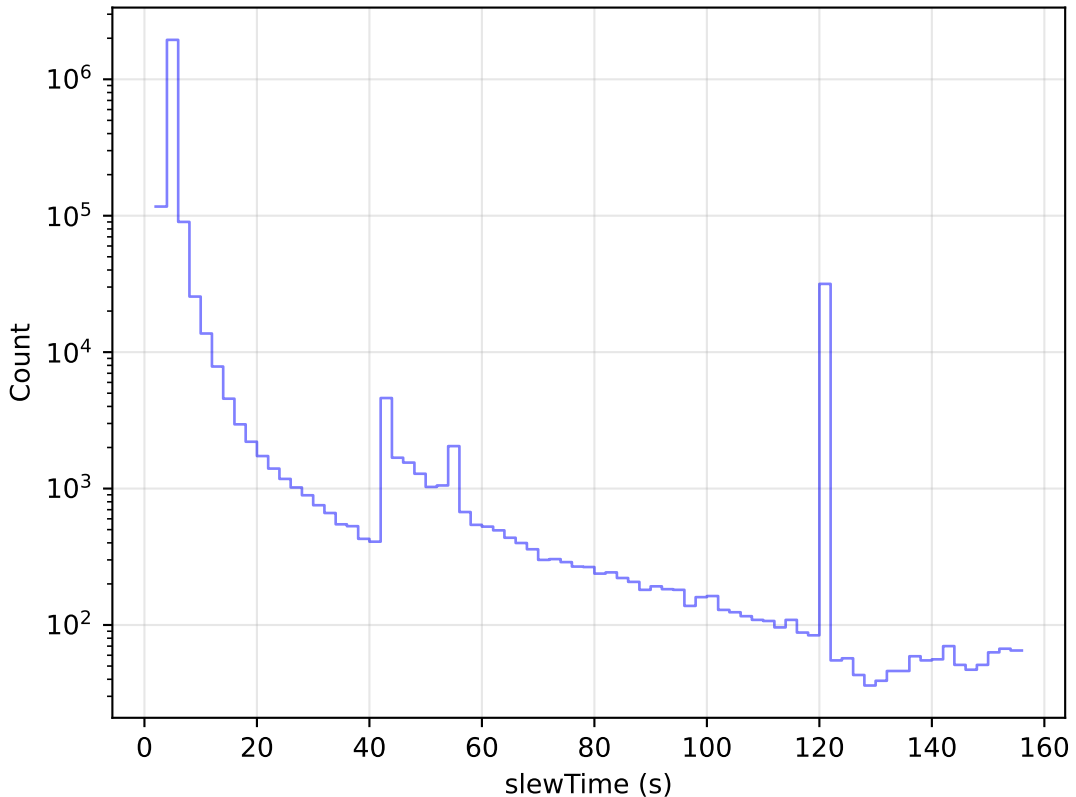
weather_cloudso18v3.4_10yrs All visits: Slew Time Histogram
