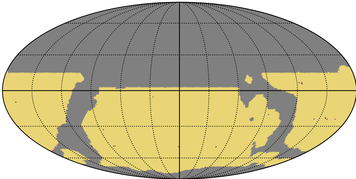
weather_cloudso18v3.4_10yrs WFD: RapidRevisits
