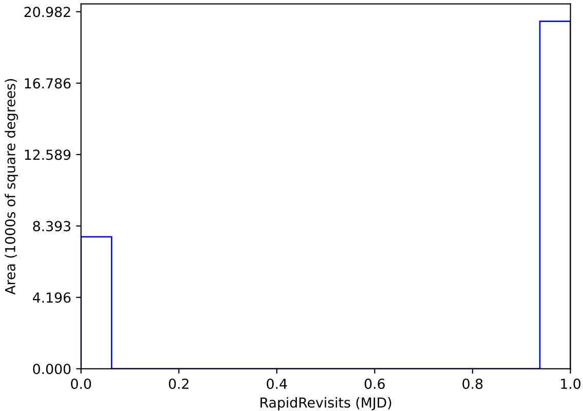
weather_cloudso18v3.4_10yrs All sky: RapidRevisits
