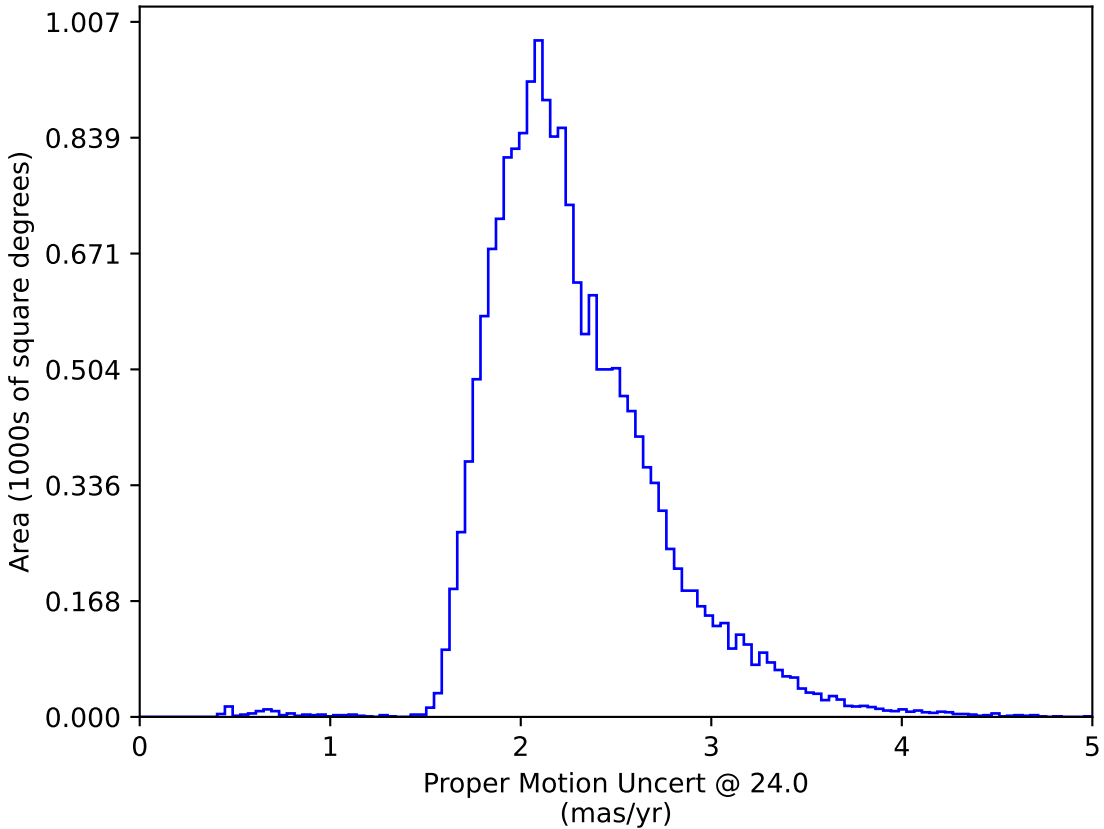
weather_cloudso18v3.4_10yrs WFD: Proper Motion Uncert @ 24.0
