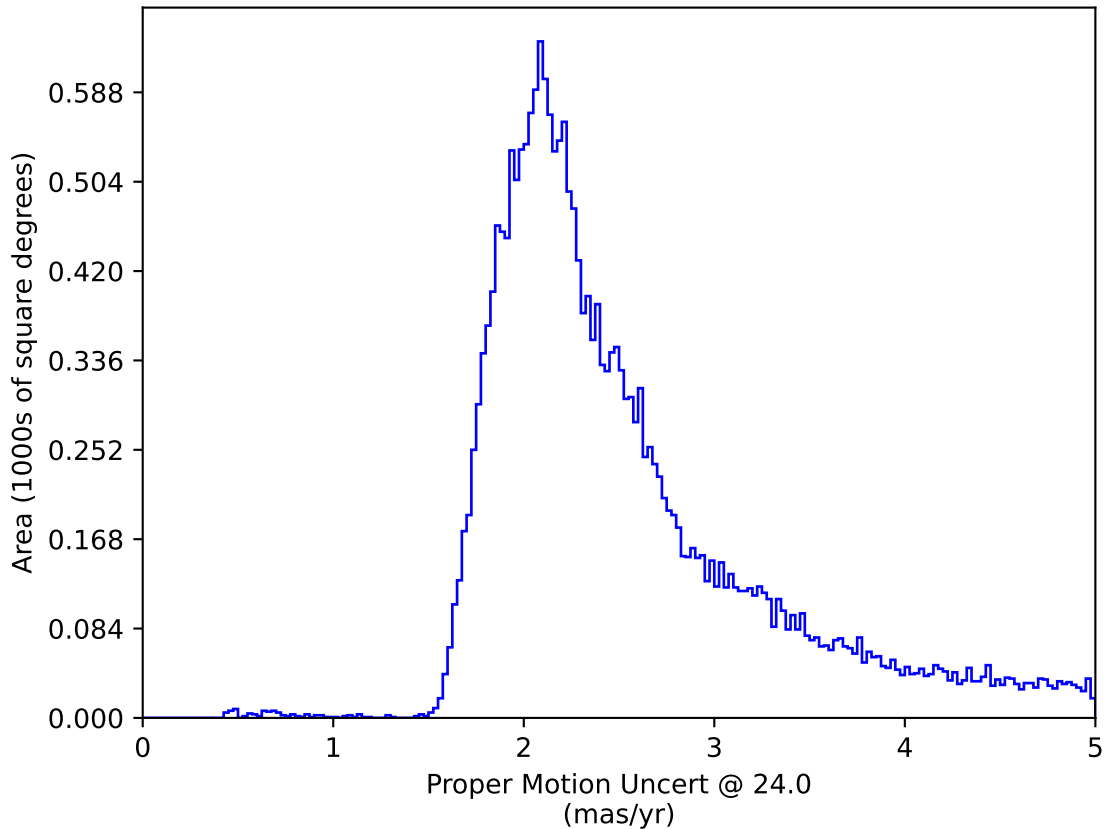
weather_cloudso18v3.4_10yrs All sky: Proper Motion Uncert @ 24.0
