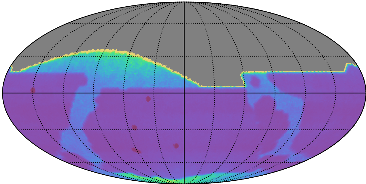
weather_cloudso18v3.4_10yrs All sky: Proper Motion Uncert @ 20.5
