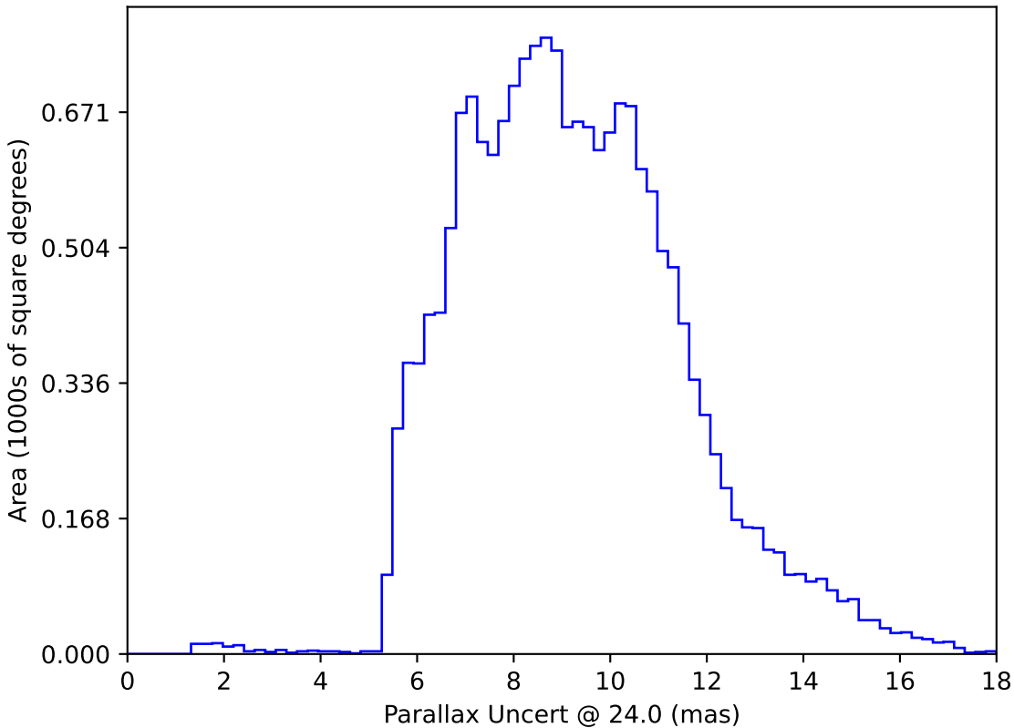
weather_cloudso18v3.4_10yrs WFD: Parallax Uncert @ 24.0
