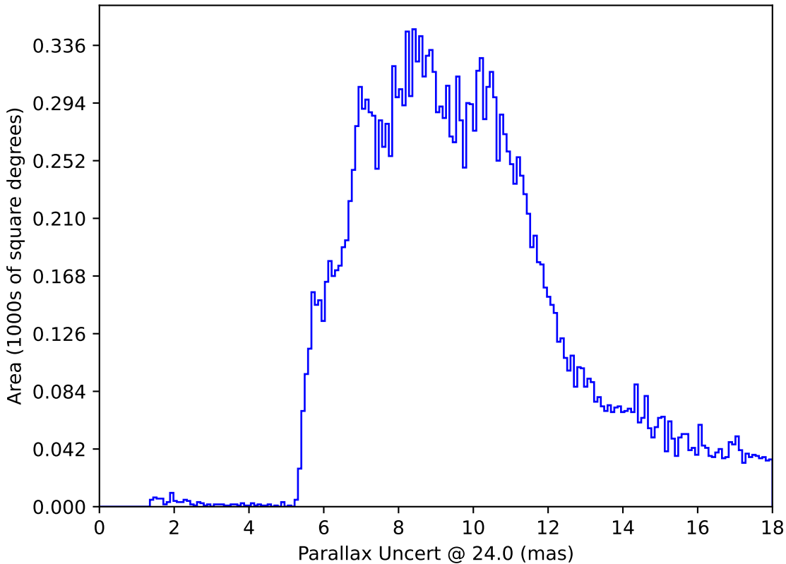
weather_cloudso18v3.4_10yrs All sky: Parallax Uncert @ 24.0
