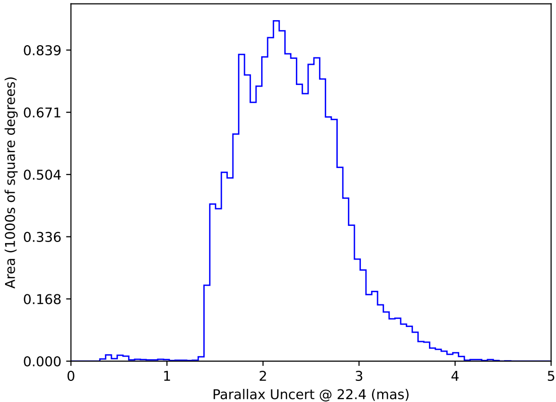
weather_cloudso18v3.4_10yrs WFD: Parallax Uncert @ 22.4
