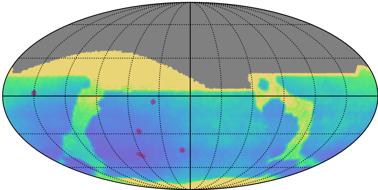
weather_cloudso18v3.4_10yrs All sky: Parallax Uncert @ 22.4
