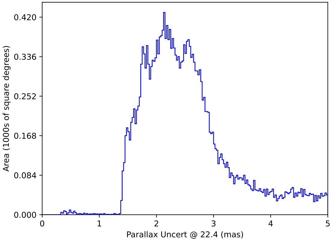
weather_cloudso18v3.4_10yrs All sky: Parallax Uncert @ 22.4
