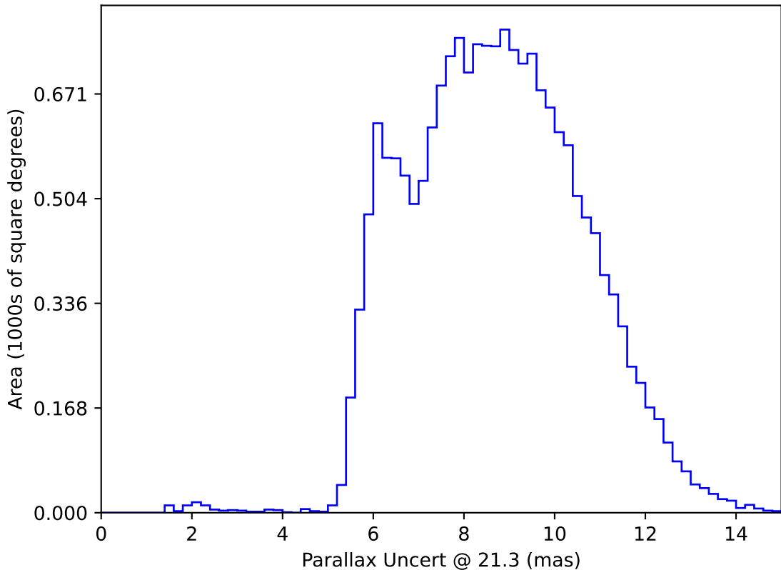
weather_cloudso18v3.4_10yrs WFD y band only: Parallax Uncert @ 21.3
