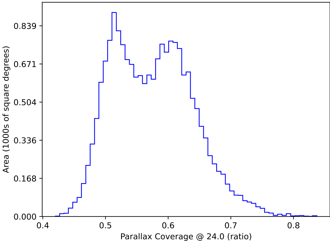
weather_cloudso18v3.4_10yrs WFD: Parallax Coverage @ 24.0
