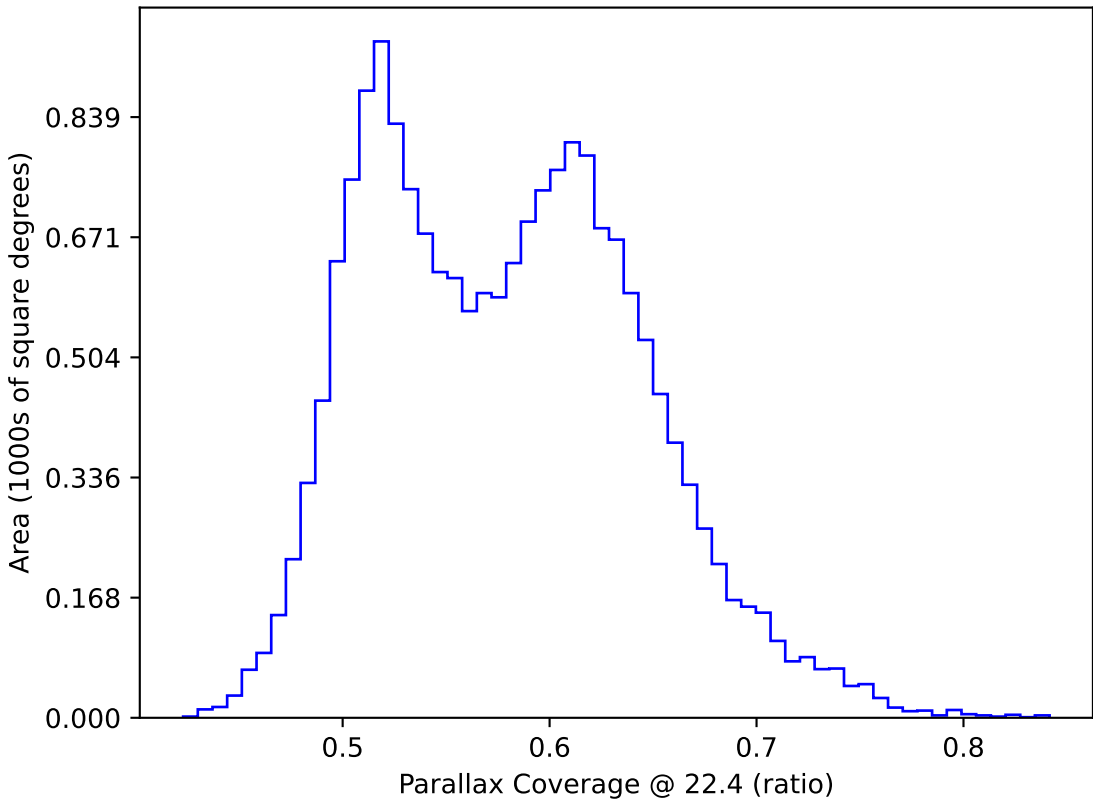
weather_cloudso18v3.4_10yrs WFD: Parallax Coverage @ 22.4
