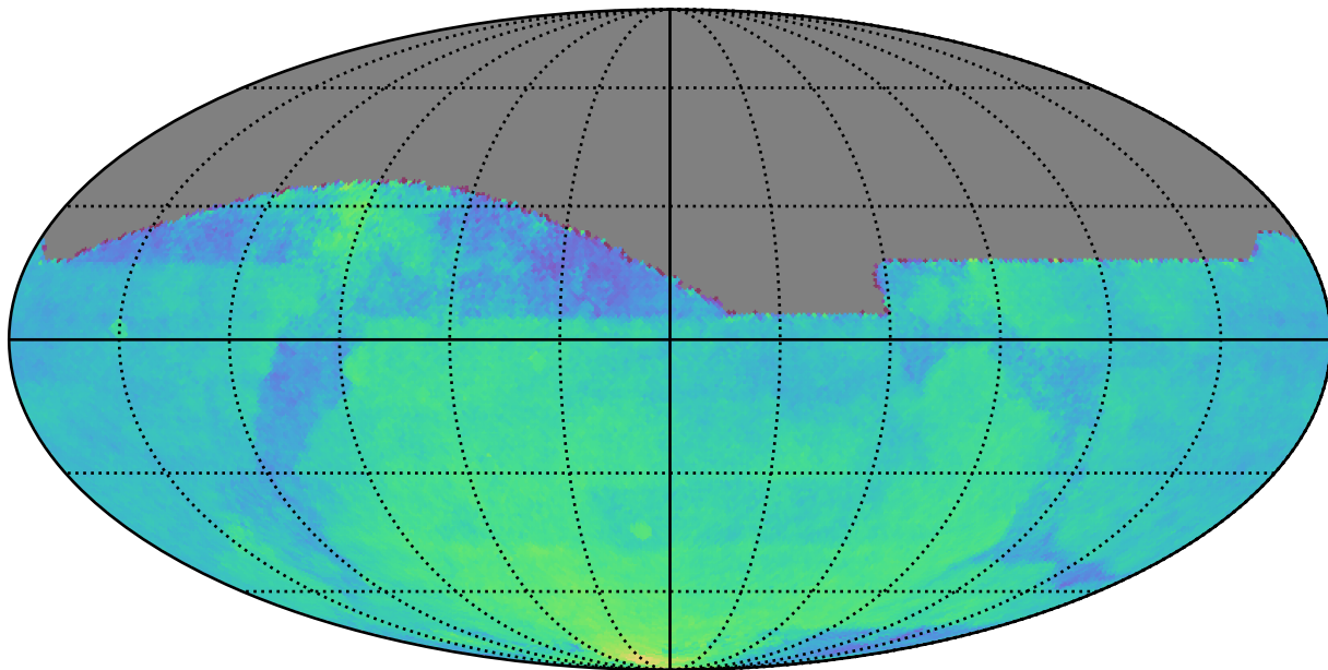
weather_cloudso18v3.4_10yrs All sky: Parallax Coverage @ 22.4
