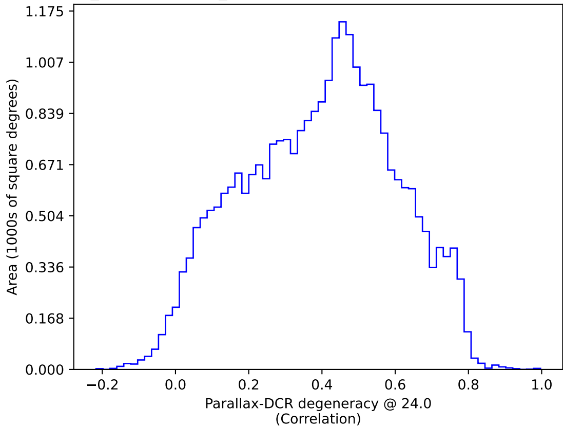
weather_cloudso18v3.4_10yrs All sky: Parallax-DCR degeneracy @ 24.0
