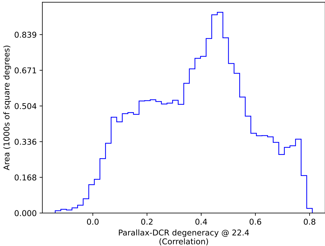
weather_cloudso18v3.4_10yrs WFD: Parallax-DCR degeneracy @ 22.4
