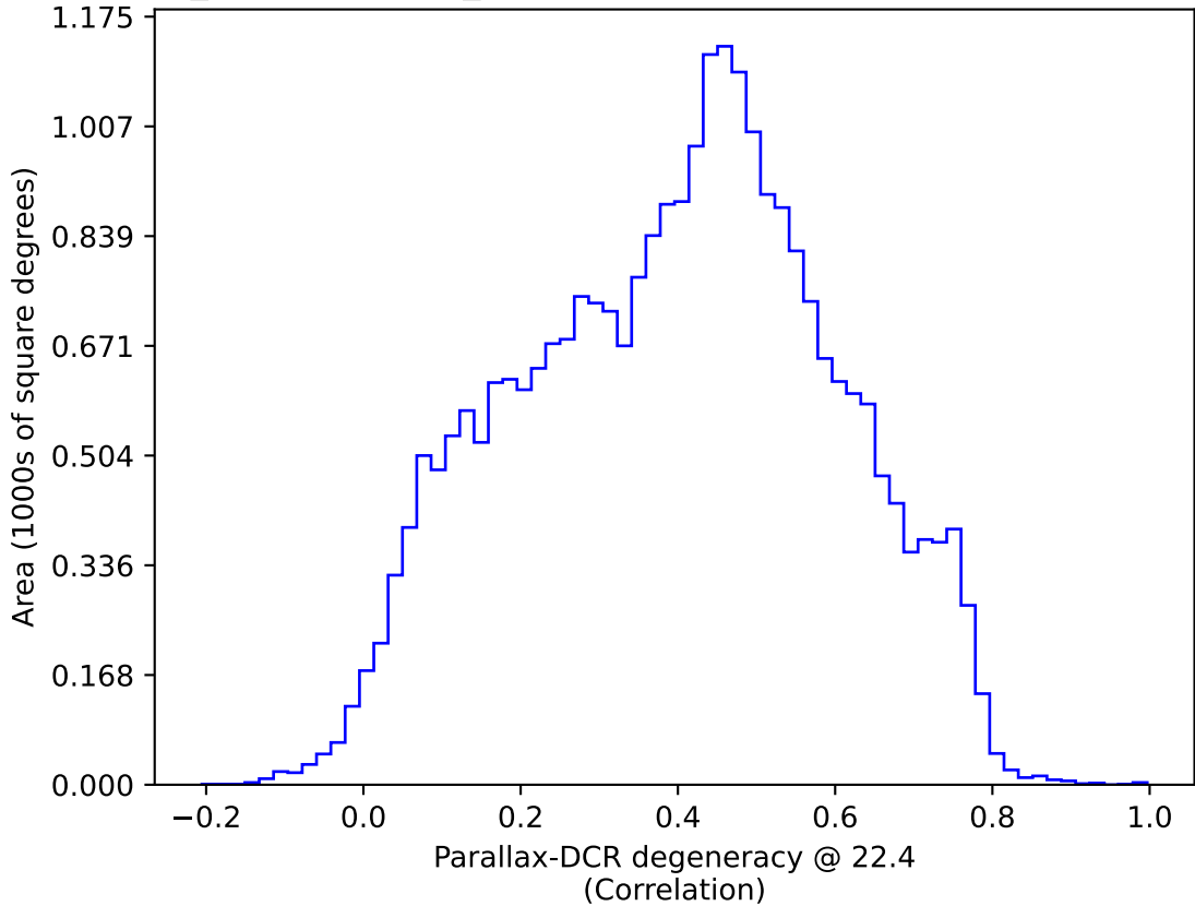
weather_cloudso18v3.4_10yrs All sky: Parallax-DCR degeneracy @ 22.4
