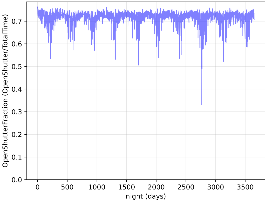
weather_cloudso18v3.4_10yrs Per night: OpenShutterFraction
