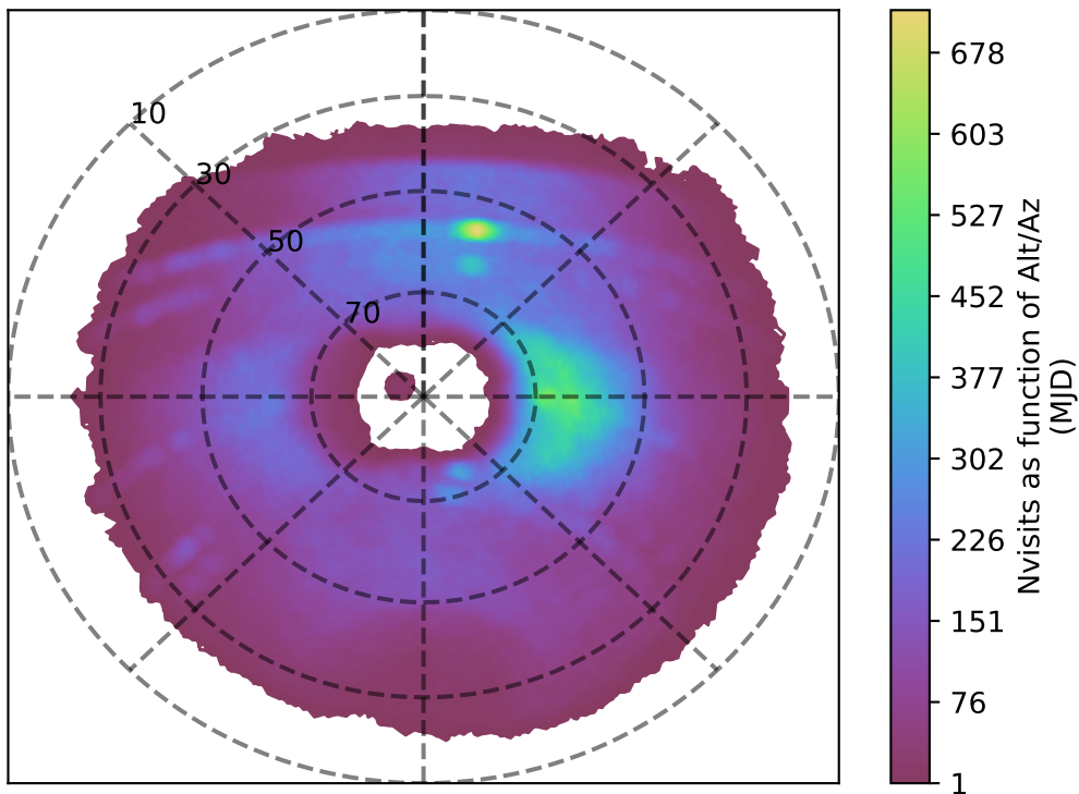
weather_cloudso18v3.4_10yrs u band: Nvisits as function of Alt/Az
