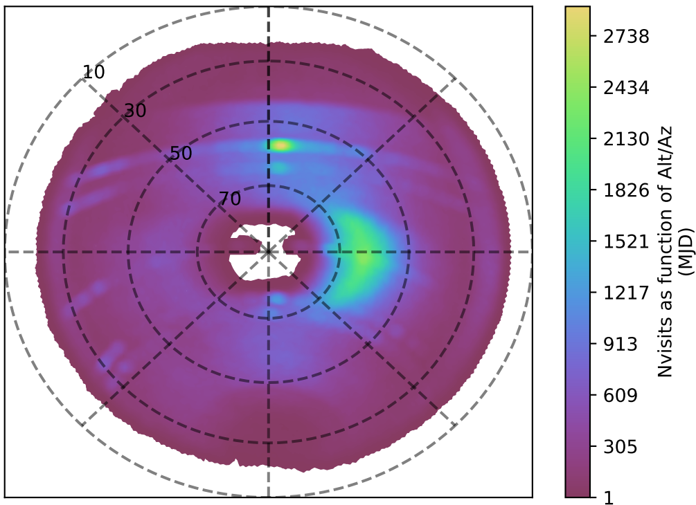
weather_cloudso18v3.4_10yrs i band: Nvisits as function of Alt/Az
