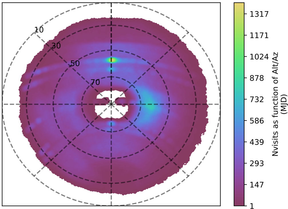
weather_cloudso18v3.4_10yrs g band: Nvisits as function of Alt/Az
