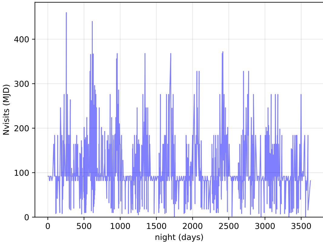
weather_cloudso18v3.4_10yrs DDF: Nvisits
