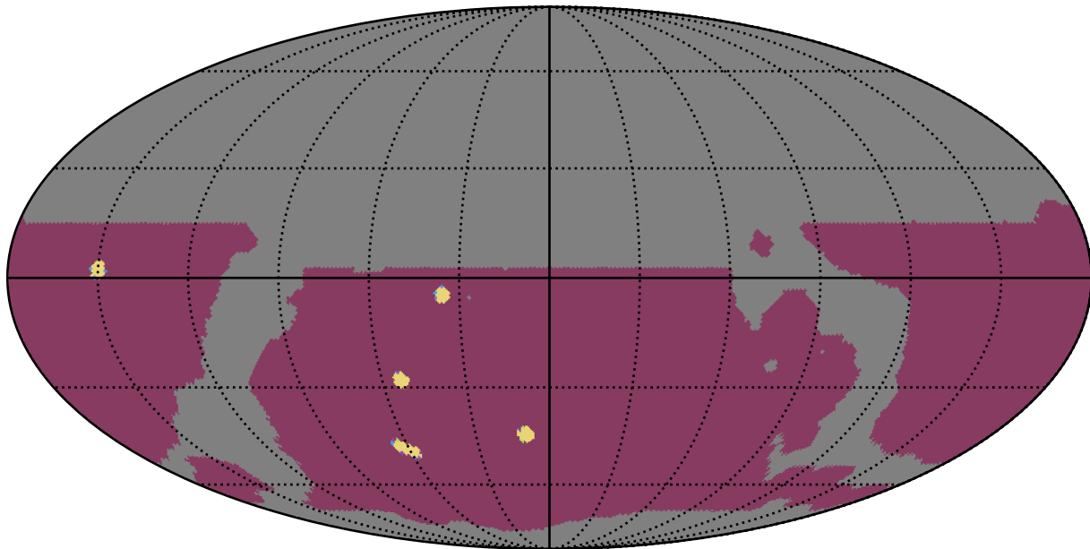
weather_cloudso18v3.4_10yrs WFD: NumberOfQuickRevisits
