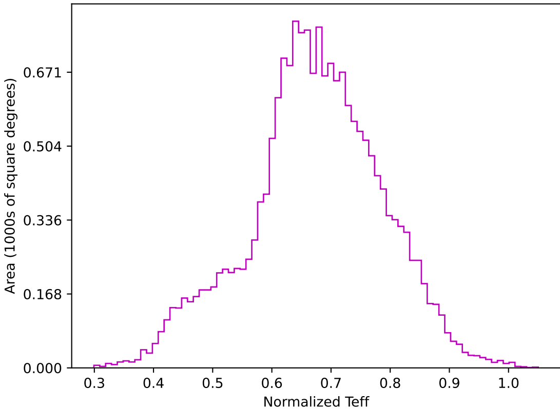
weather_cloudso18v3.4_10yrs WFD z band: Normalized Teff
