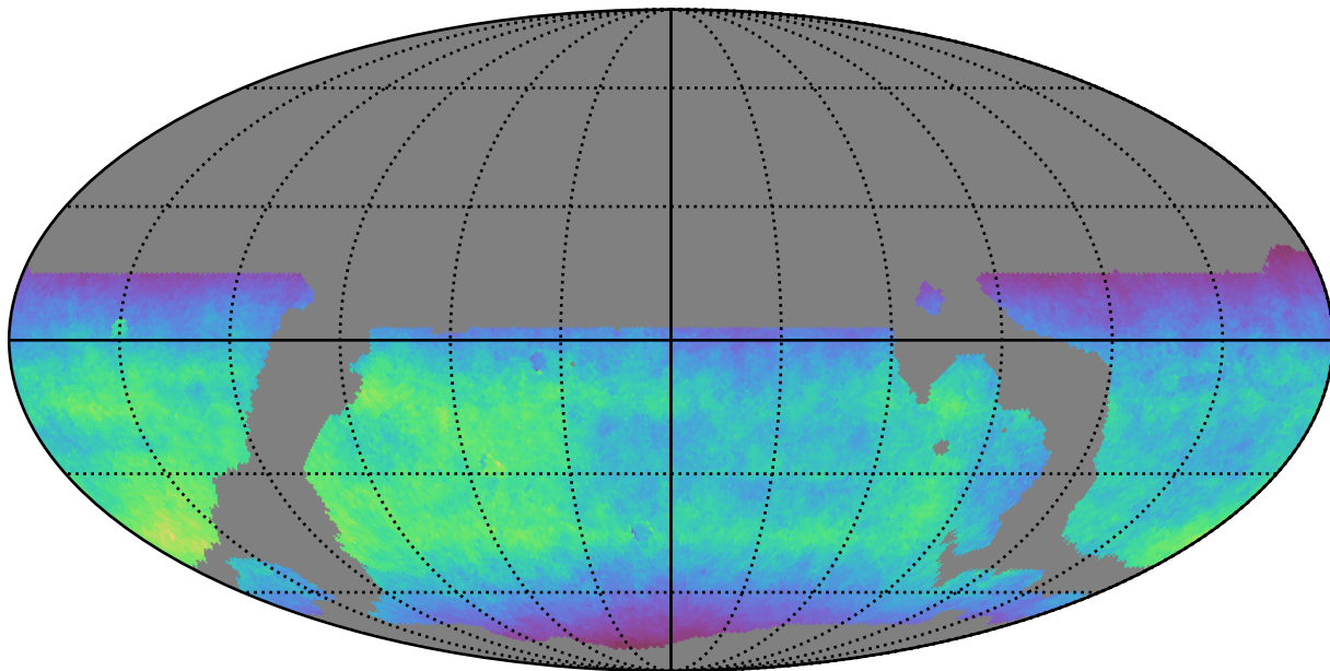
weather_cloudso18v3.4_10yrs WFD y band: Normalized Teff
