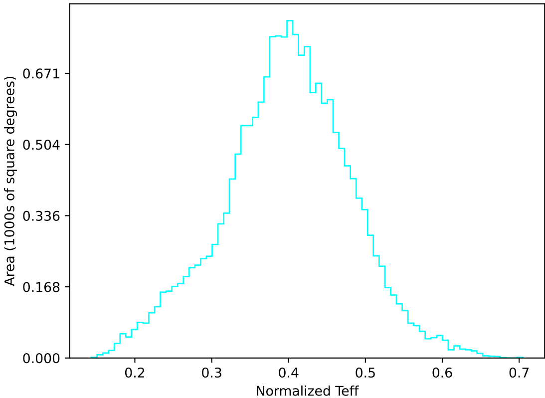
weather_cloudso18v3.4_10yrs WFD u band: Normalized Teff
