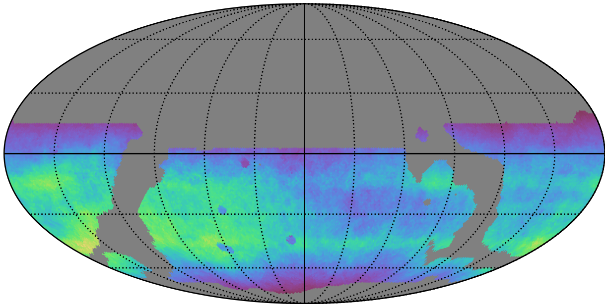
weather_cloudso18v3.4_10yrs WFD r band: Normalized Teff
