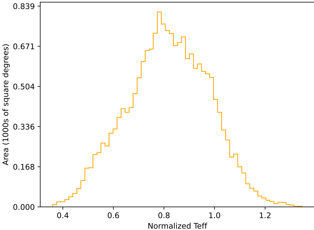
weather_cloudso18v3.4_10yrs WFD r band: Normalized Teff
