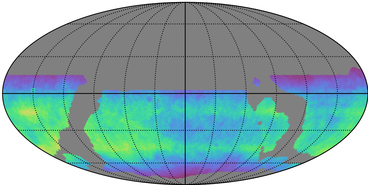
weather_cloudso18v3.4_10yrs WFD i band: Normalized Teff
