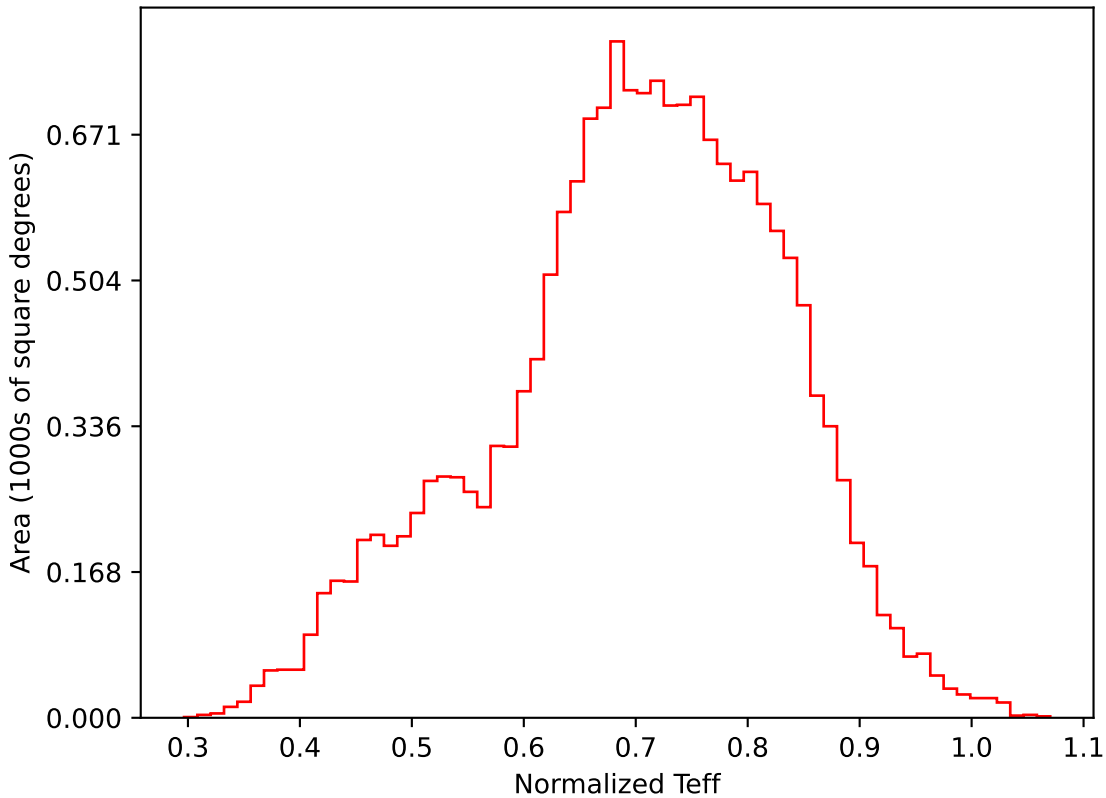
weather_cloudso18v3.4_10yrs WFD i band: Normalized Teff
