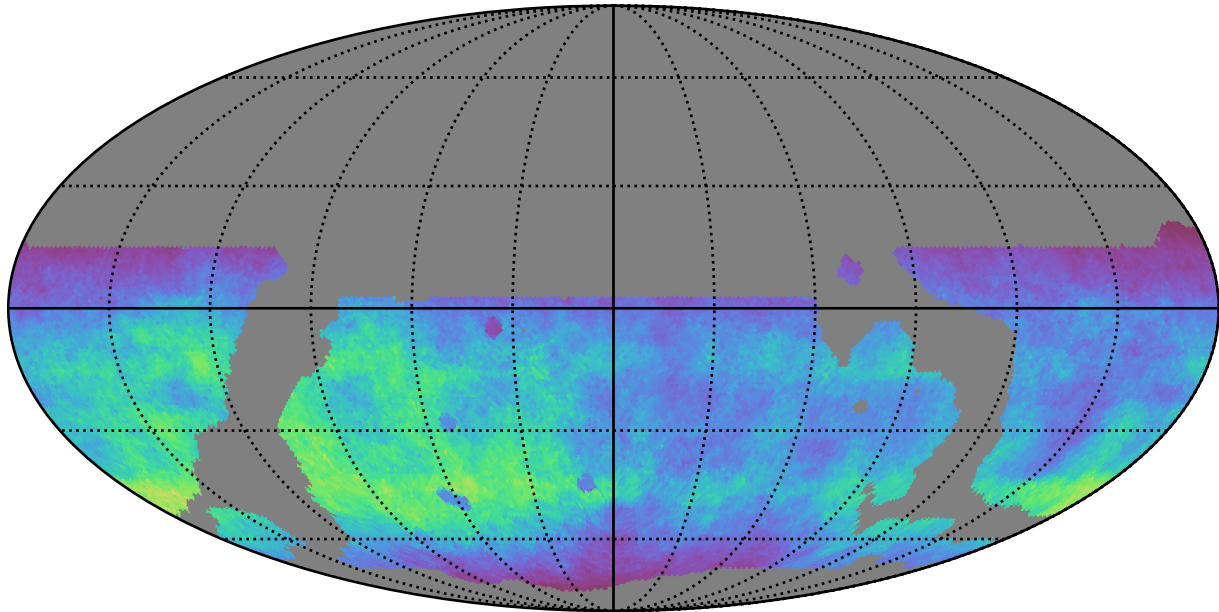
weather_cloudso18v3.4_10yrs WFD g band: Normalized Teff
