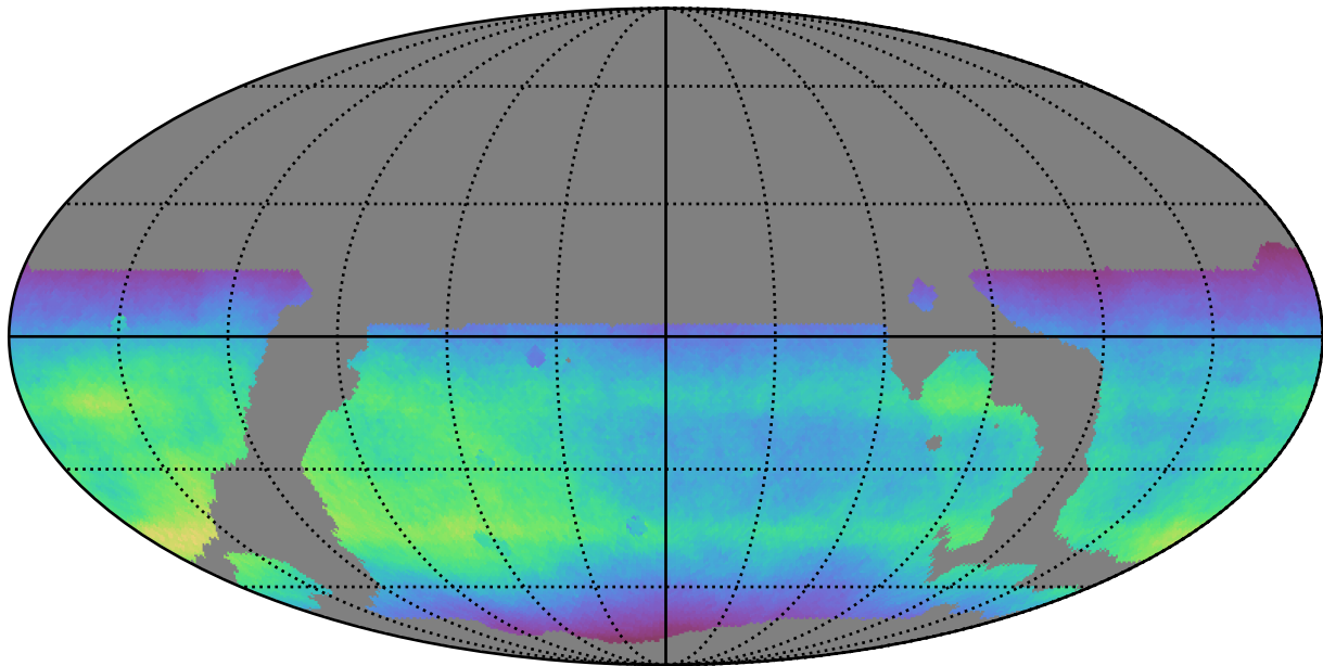
weather_cloudso18v3.4_10yrs WFD all bands: Normalized Teff
