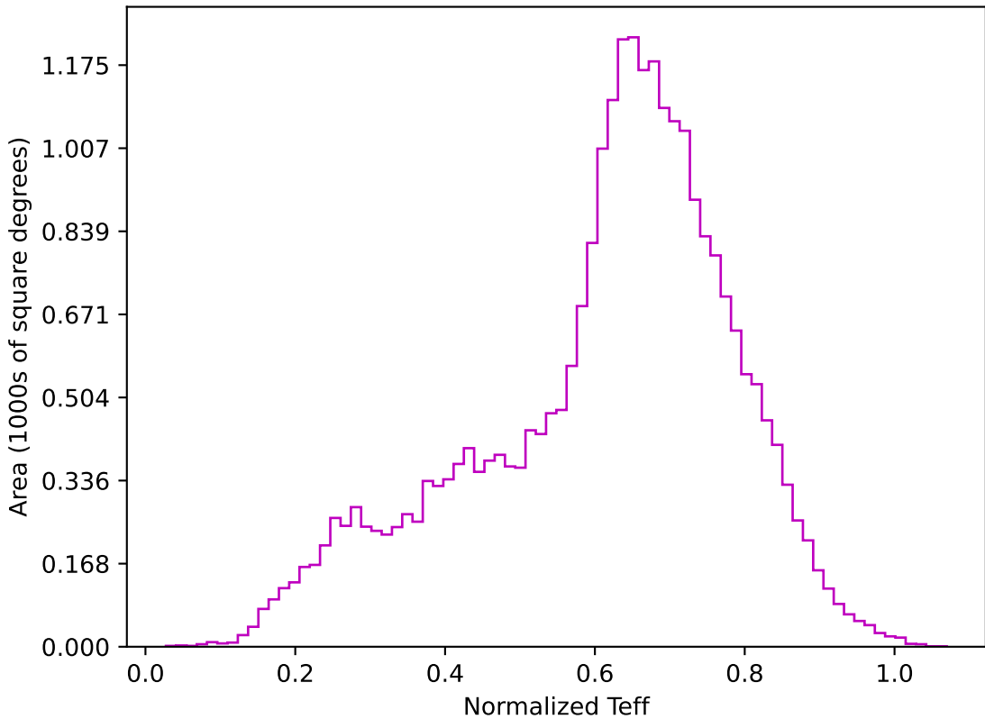
weather_cloudso18v3.4_10yrs All sky z band: Normalized Teff
