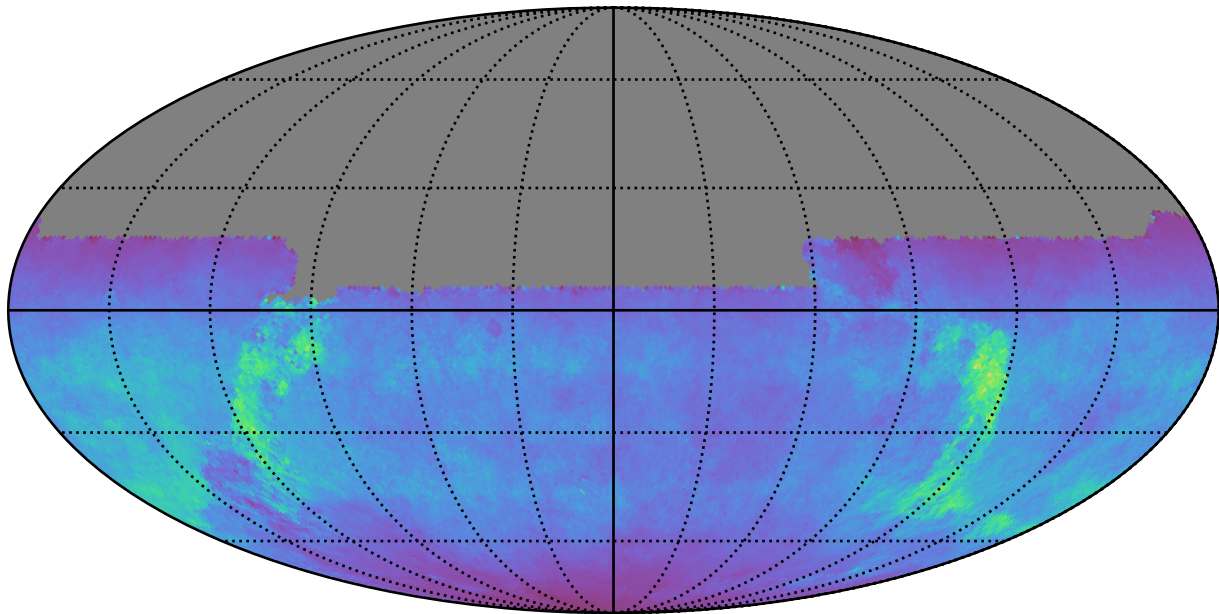
weather_cloudso18v3.4_10yrs All sky u band: Normalized Teff
