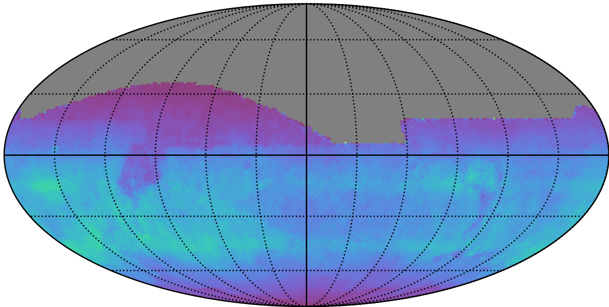
weather_cloudso18v3.4_10yrs All sky i band: Normalized Teff
