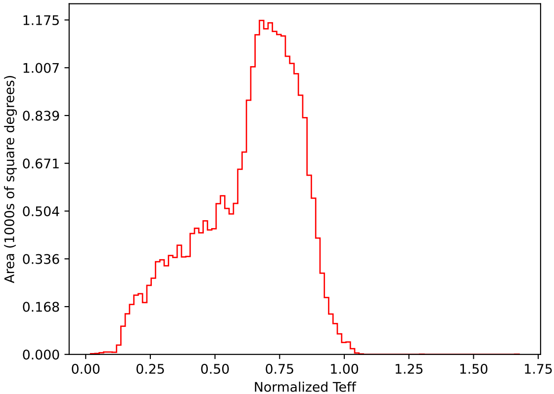
weather_cloudso18v3.4_10yrs All sky i band: Normalized Teff
