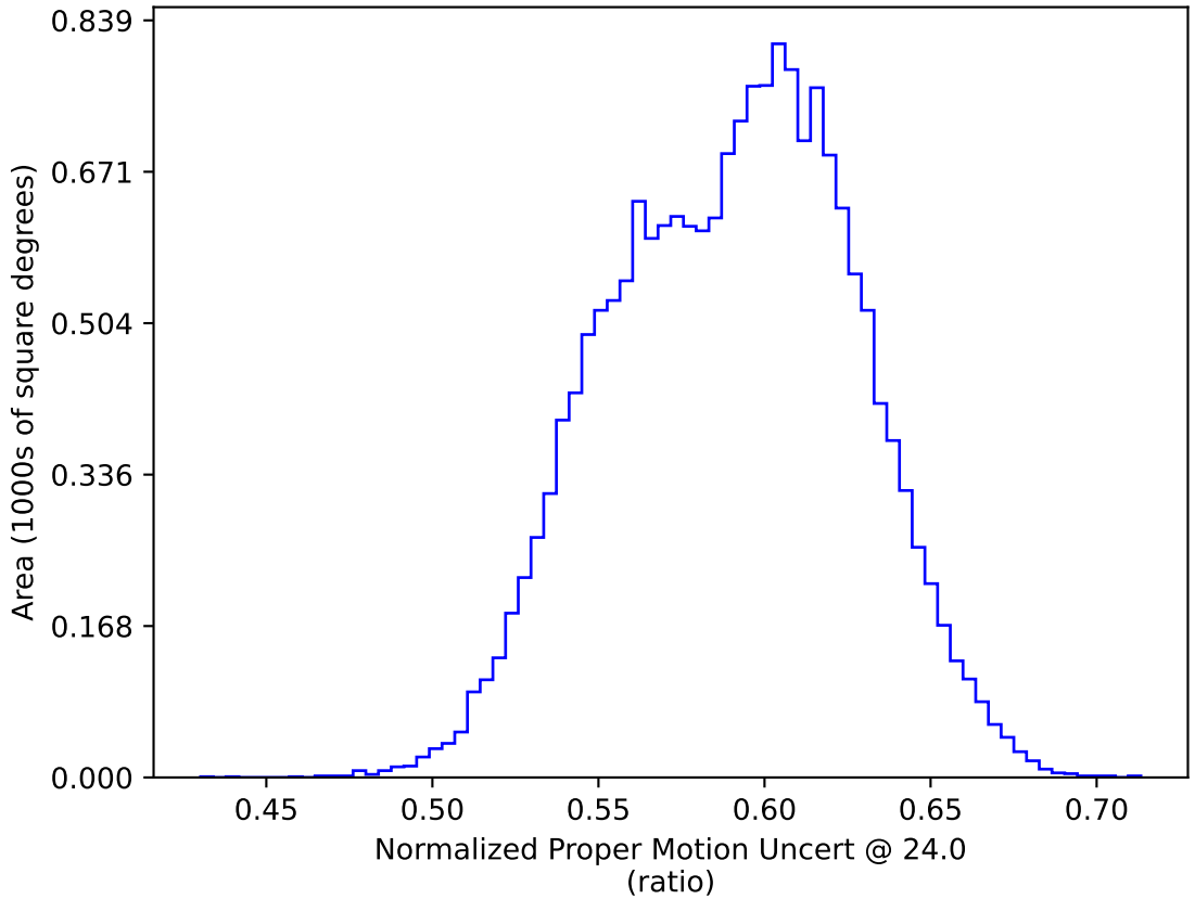
weather_cloudso18v3.4_10yrs WFD: Normalized Proper Motion Uncert @ 24.0
