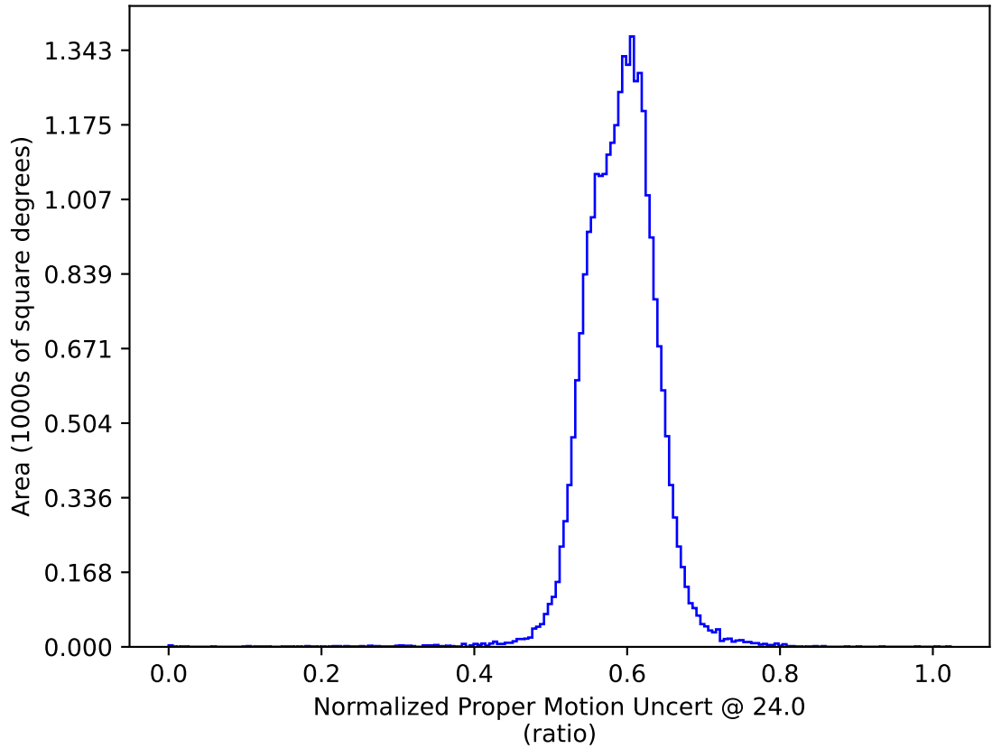
weather_cloudso18v3.4_10yrs All sky: Normalized Proper Motion Uncert @ 24.0
