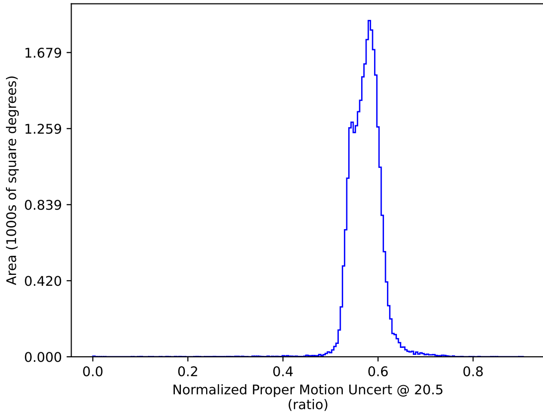
weather_cloudso18v3.4_10yrs All sky: Normalized Proper Motion Uncert @ 20.5
