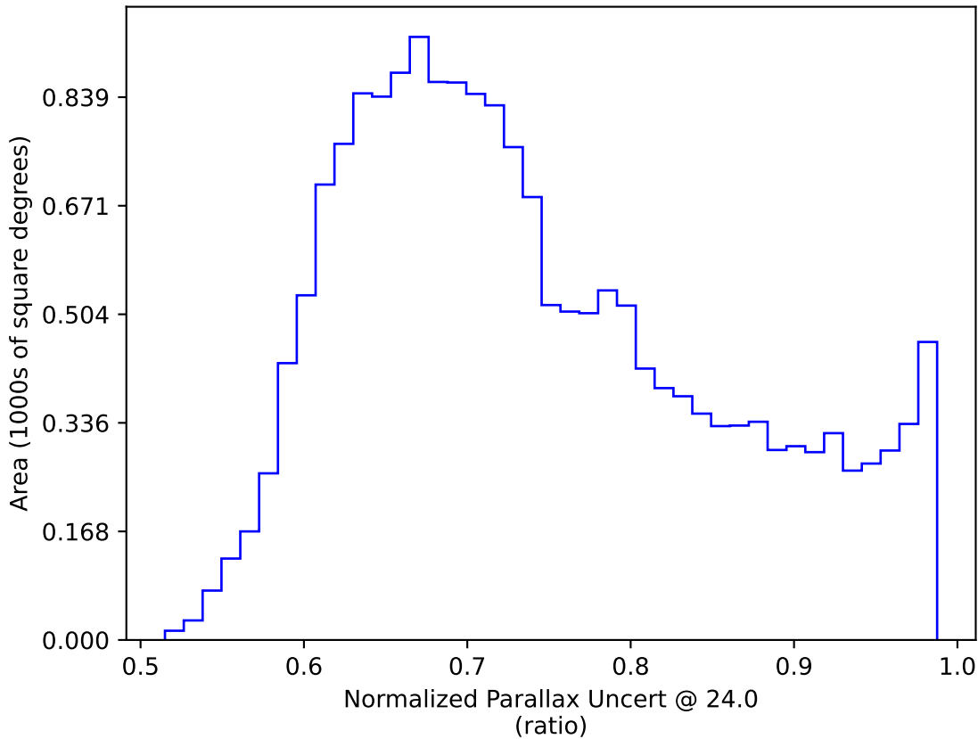
weather_cloudso18v3.4_10yrs WFD: Normalized Parallax Uncert @ 24.0
